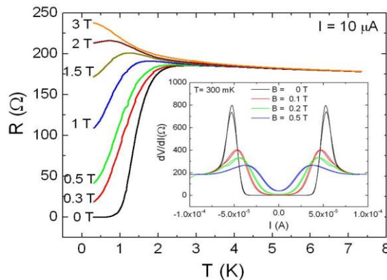
Superconducting nanodiamond films (left) Calculated DOS show the gap for various levels of disorder. (right) Superconductor-insulator transition in nanodiamond. Inset: Differential resistance curve shows a superconducting gap at low B and T .
