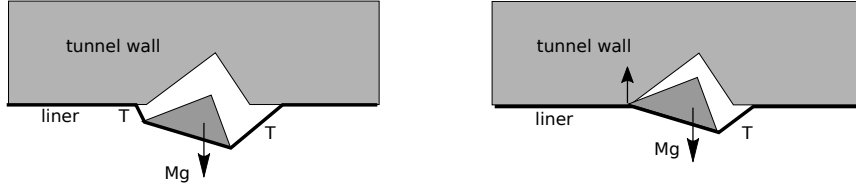
Figure 7: Attached and unattached rock held in place by a liner.
