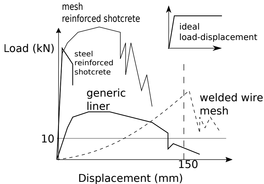
Figure 3: Load versus displacement (pull tests) curves for various wall support procedures, including a generic TSL liner. An ideal load-displacement is also indicated. Taken from Tannant [4].
