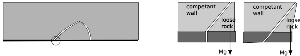
Figure 5: Failure through liner rupture. Left: The supported rock. Right: A close up of the situation near the rupture point (circle). Two liner rupture modes are possible: shear failure and tensile failure.
